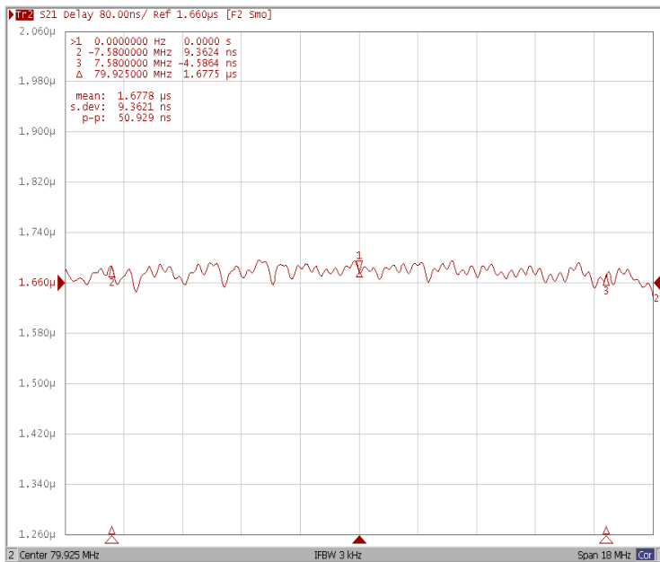
Group Delay Variation Fo±7.58MHz
